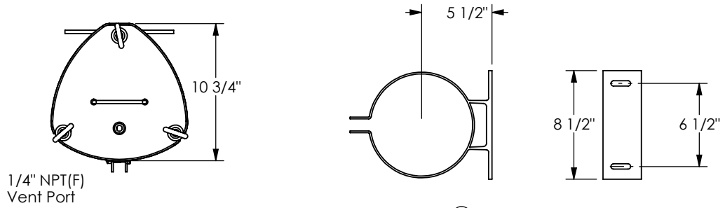
(B) 79-0938 Ring Bracket
