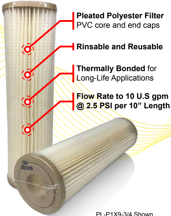
PL-P1X9-3/4 Shown.
